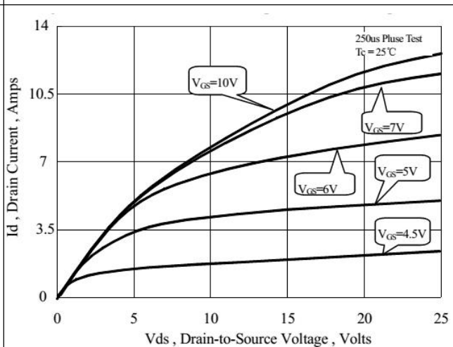
Figure 6. On-State Characteristics
